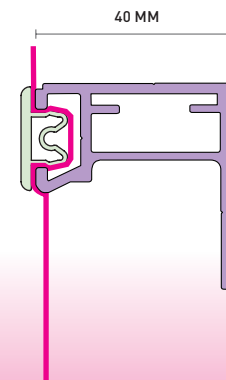
NOV 432 NOVASKIN TRIM ADAPTER
