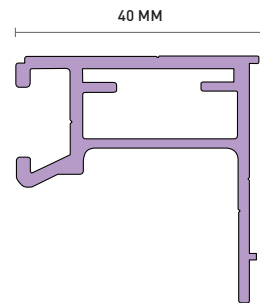
NOV 431 NOVASKIN FRAME
