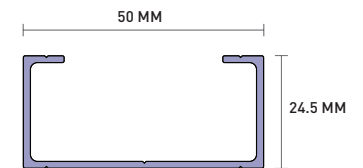
NOV 103 STANDARD SUPPORT
