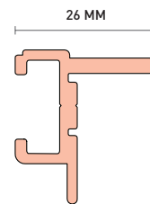
NOV 432 NOVASKIN TRIM ADAPTER
